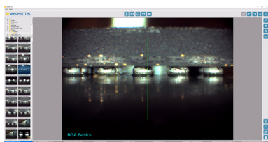
BGA bumps (large field of view)
