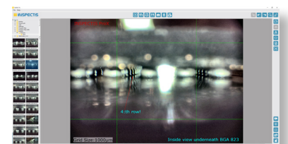
Inner rows of BGA bumps
