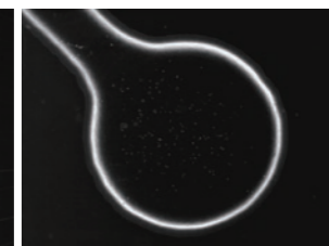
High density PCB Darkfield illumination at optical magnification 16x
